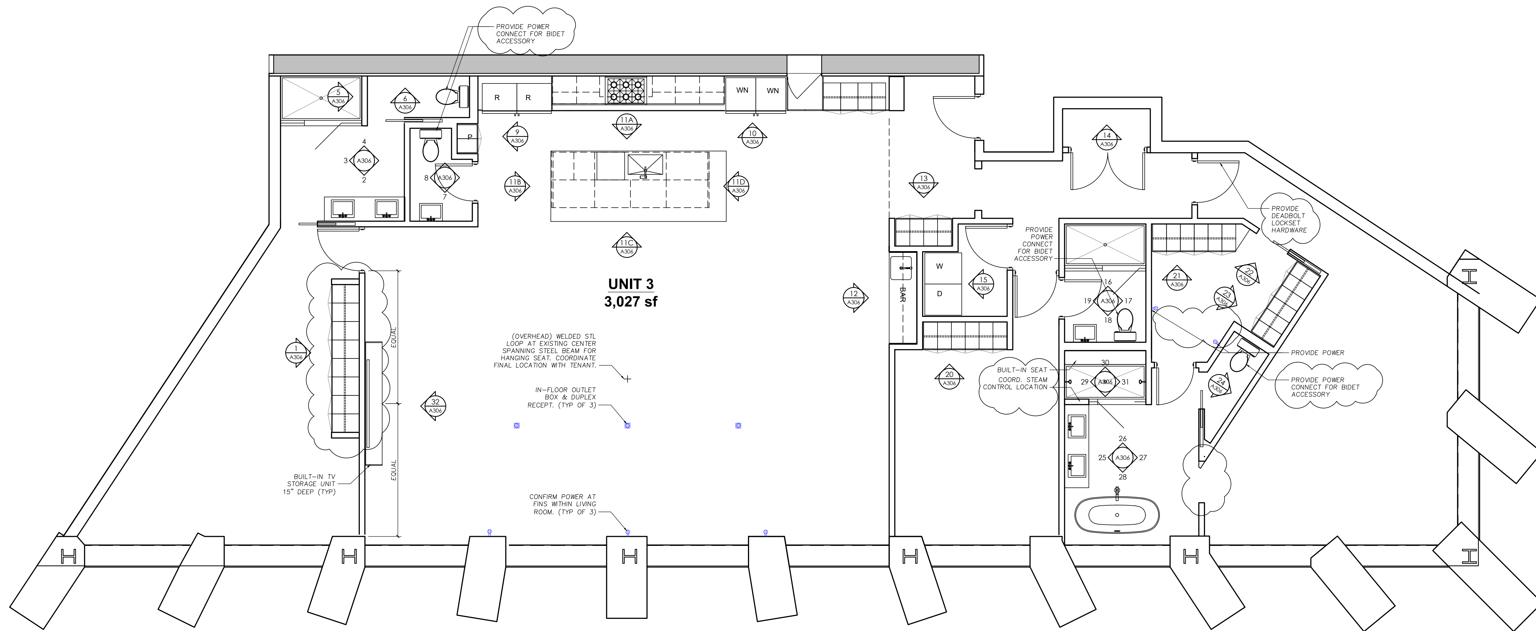
1 ENLARGED PLAN - UNIT 3 SCALE: 1/4" = 1'-0"
